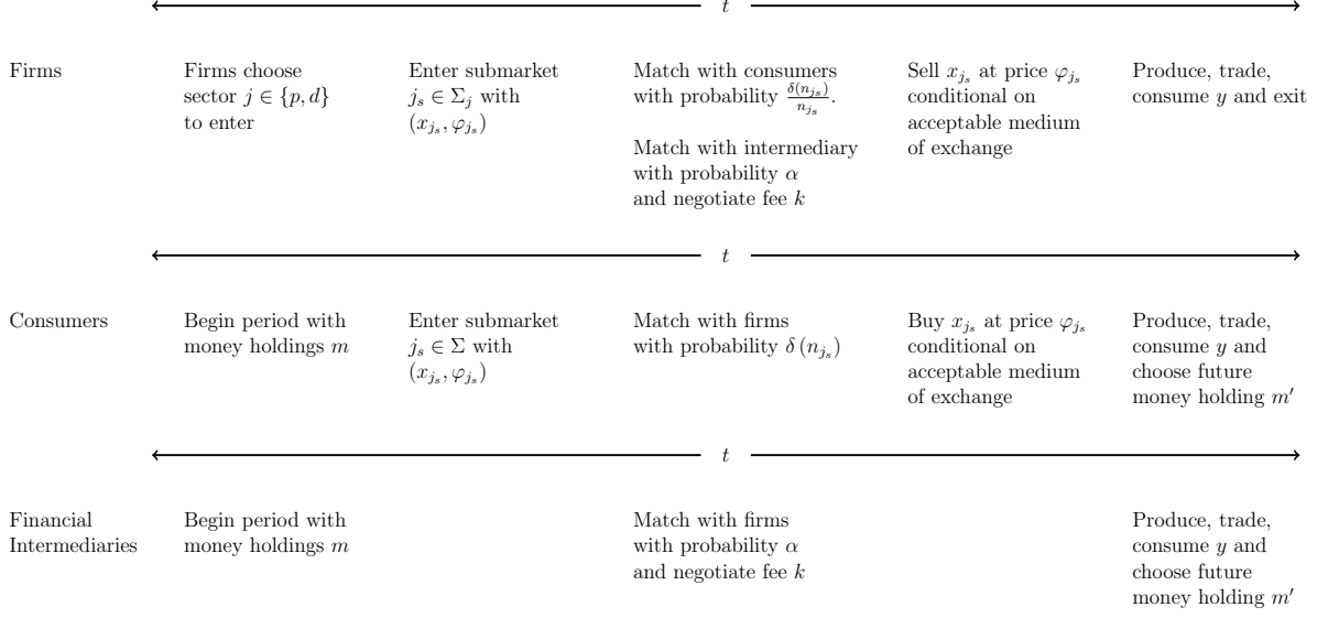
Figure 3: Model Timing
